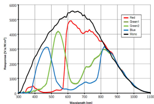
Spectral Response Curve
